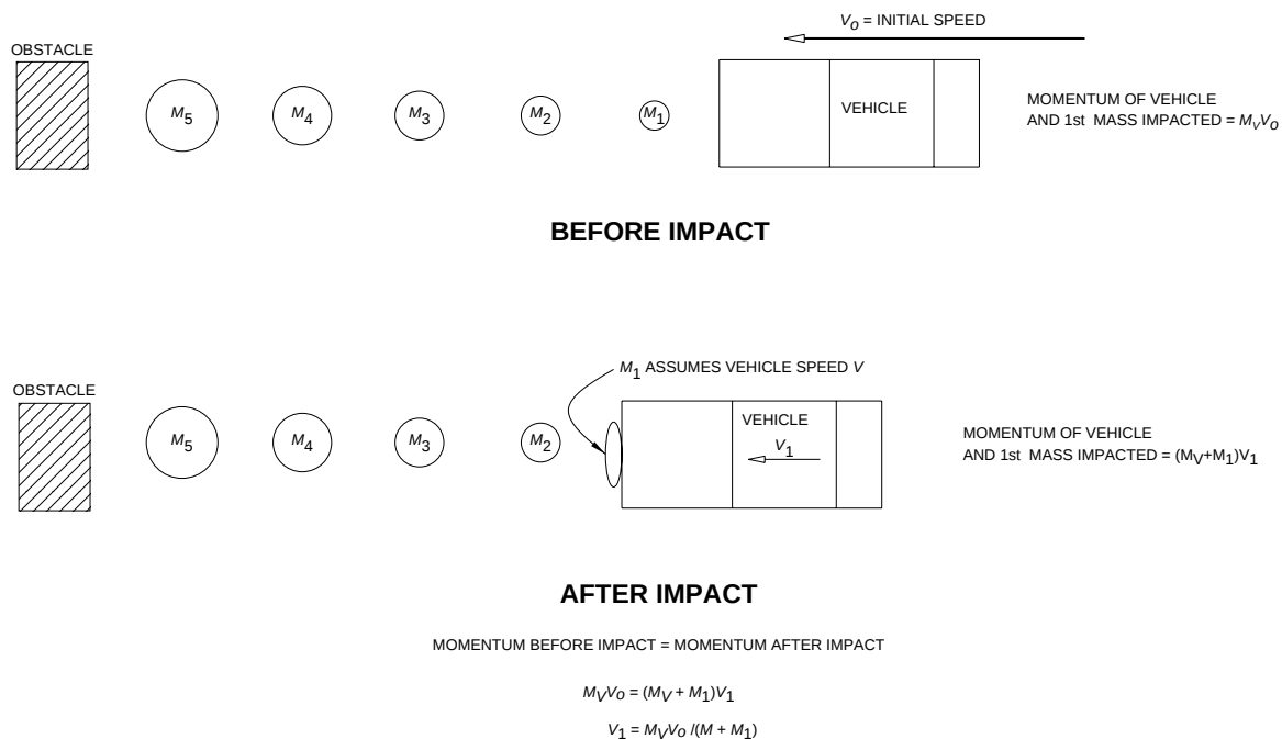
Figure 8-38. Conservation of Momentum Principle
