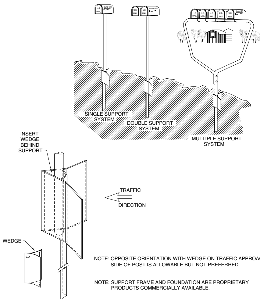
Figure 11-10. Single and Double Mailbox Assemblies, Series C
