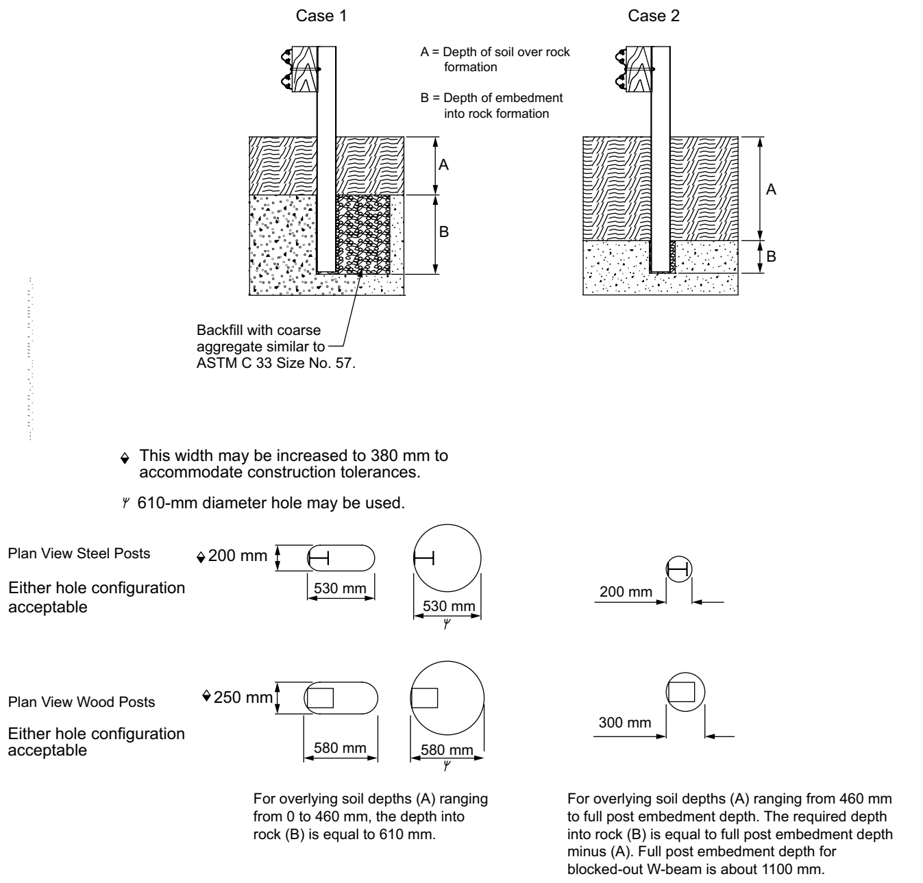
Figure 5-51(a). Guardrail Post Details in Rock Formation (Metric Units)
