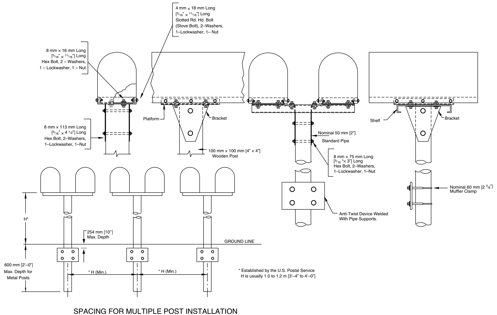
Figure 11-7. Single and Double Mailbox Assemblies, Series A
