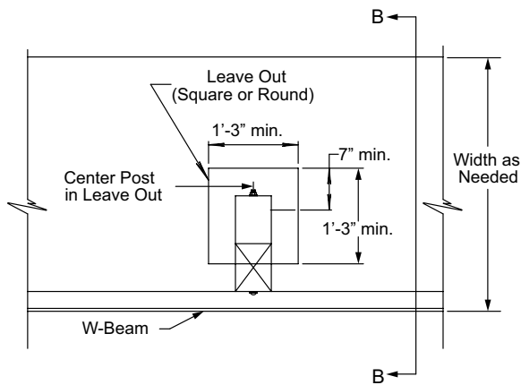
Wood Post Detail
