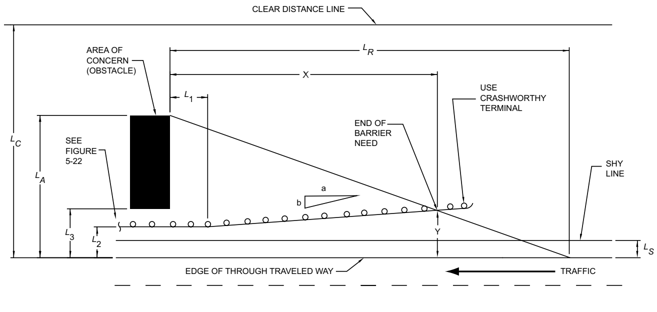
Figure 5-39. Approach Barrier Layout Variables
