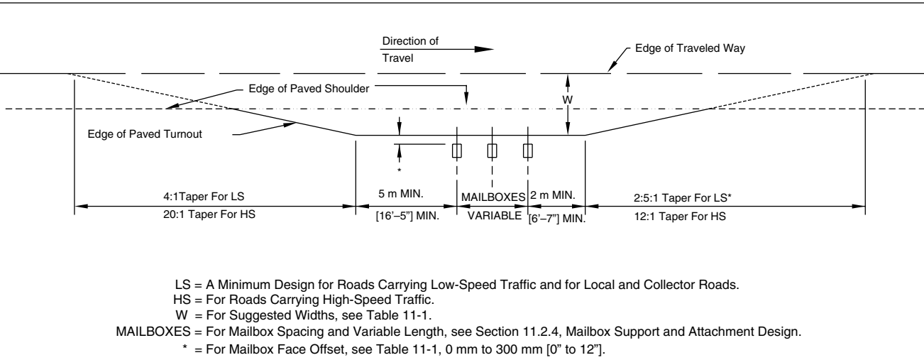
Figure 11-5. Mailbox Turnout
