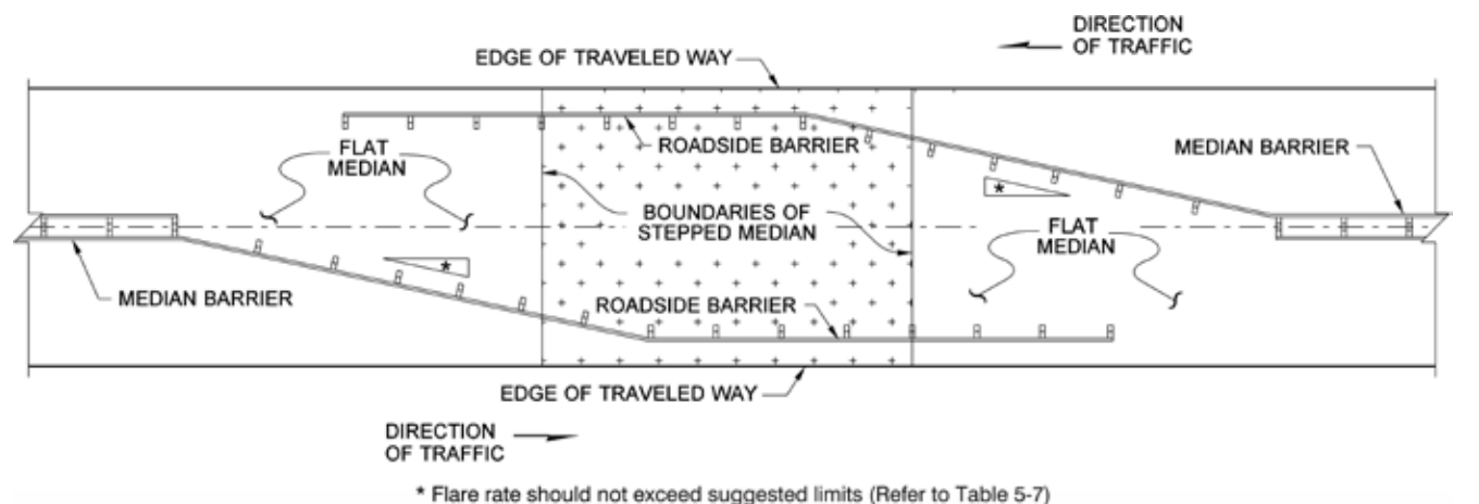
Figure 6-19. Example of a Split Median Barrier Layout
