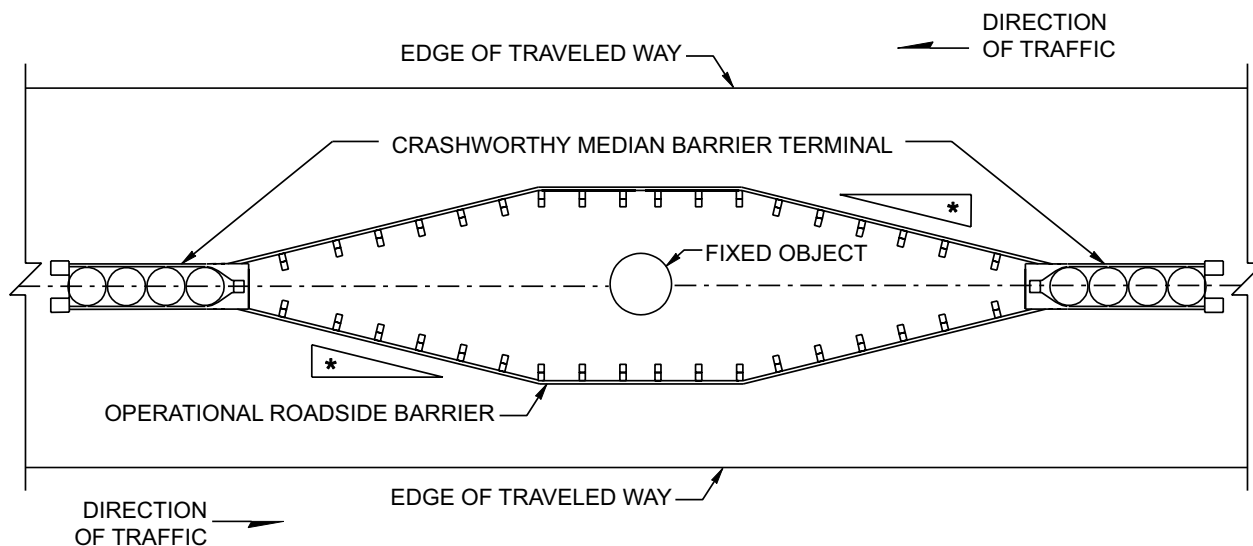
Figure 6-20. Suggested Layout for Shielding a Rigid Object in a Median
