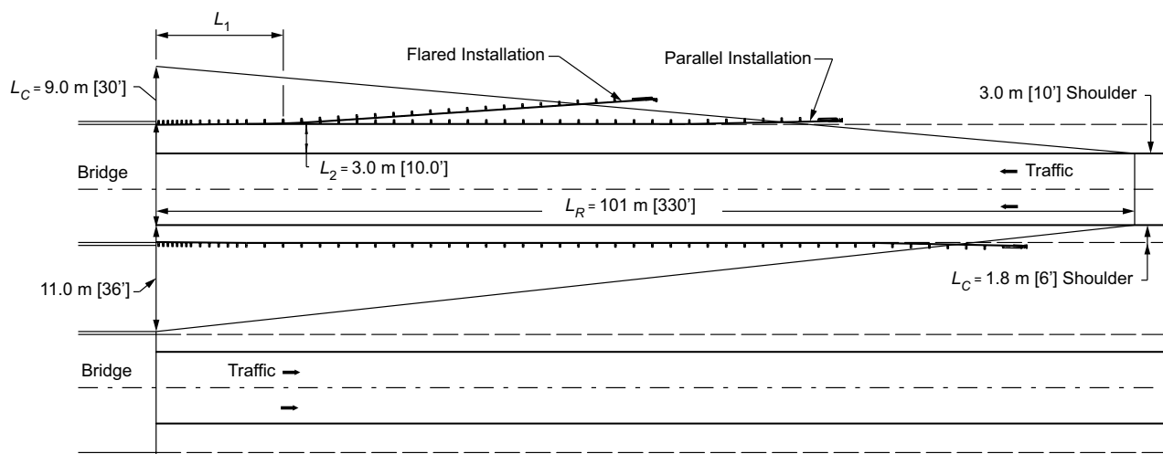
Figure 5-45. Example of Barrier Design for Bridge Approach
